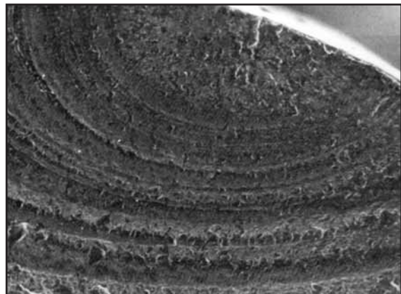
Fig. 17: The fatigue crack radiates out from the origin as a series of concentric rings (termed rest lines, beach lines or striations).
