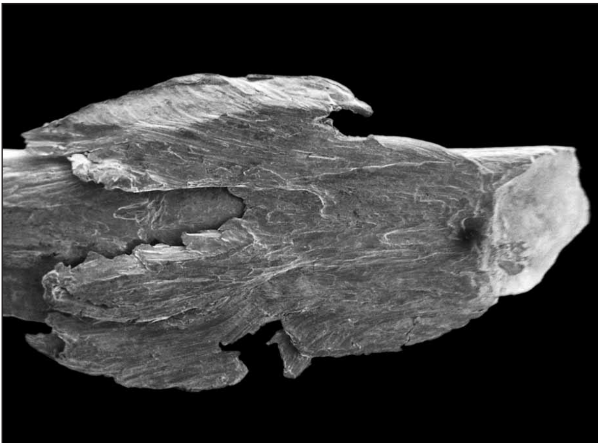
Fig. 54: Severe plastic deformation caused by the rope hitting a steel structure. The high axial line pull combined with high transverse loading, has finally lead to the shear failure of the wire.
