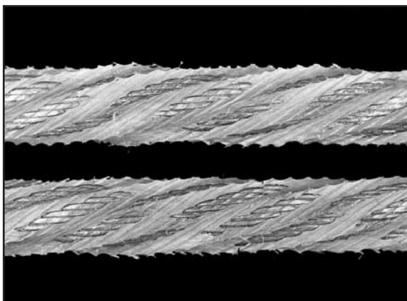
Fig. 146: An unsuited plastic material will not give sufficient support to the outer strands. It will wear and lead to premature rope failure.
