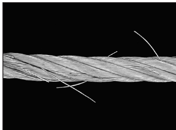
Fig. 96: Internal wire breaks are never alone. If you find one, look for more!
