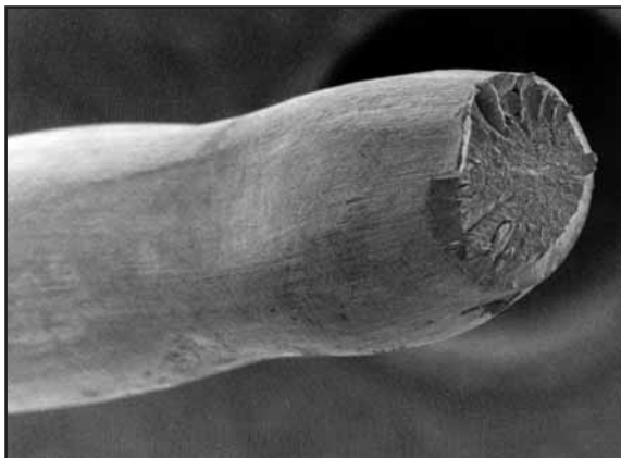
Fig. 40: Before failing by tensile overload, this wire developed two areas of local necking.
