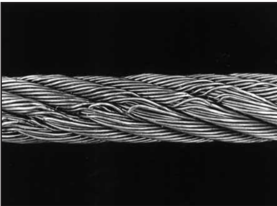
Fig. 57: An eight strand rope damaged by being dragged over the rim of a sheave. Please note the helical damage pattern.
