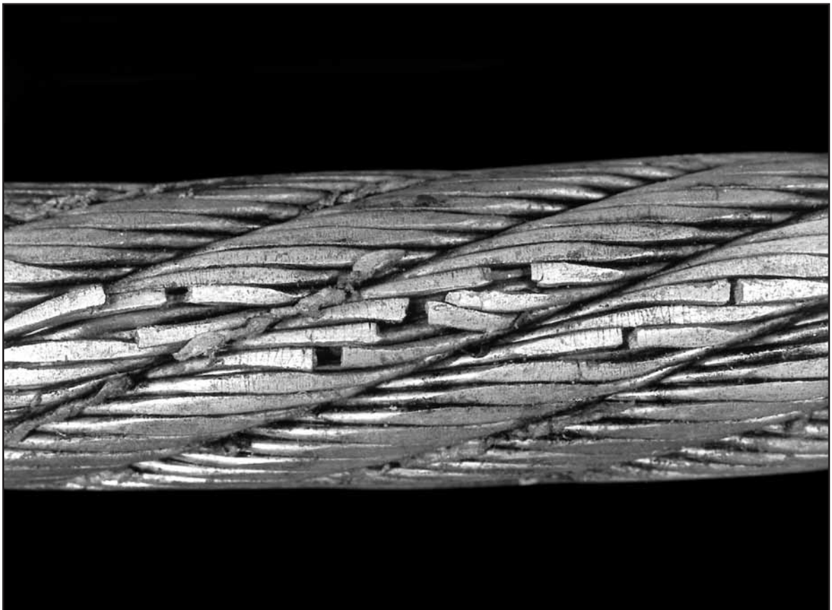
Fig. 111: This eight strand rope has worked in a tight sheave. Its internal plastic layer has prevented the formation of a birdcage, but a lot of cracks have formed in the galvanized outer wires (see also Figs. 68 and 69 from the same rope).
