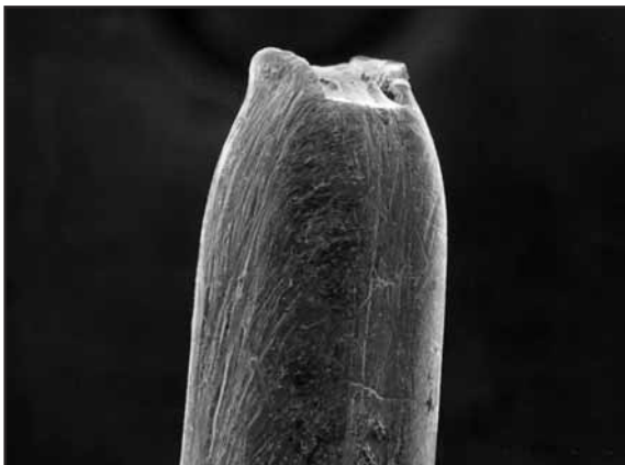
Fig. 42: Tensile overload break. If you've seen one you've seen them all.
