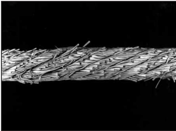
Fig. 112: This rope has been operated in a tight sheave.
