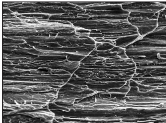
Fig. 46: An example of the microstructure of the sheared wire surface.
