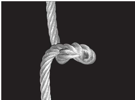
Fig. 106: The same hockle as in Fig. 105. Under load, the hockle pulls tight, causing severe rope damage.
