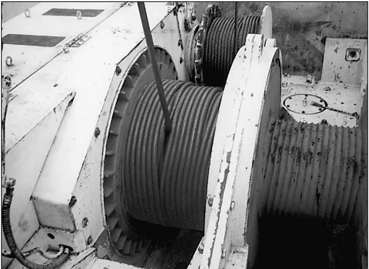
Fig. 131: This rope has been pulled into a lower, non tensioned layer during lifting. During subsequent lowering of the load, the rope got stuck and did not spool off the drum, thereby reversing the load movement.
