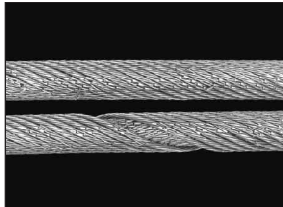
Fig. 121: This rope has operated in a groove which was much too wide, leading to premature wire failure along the line of contact.
