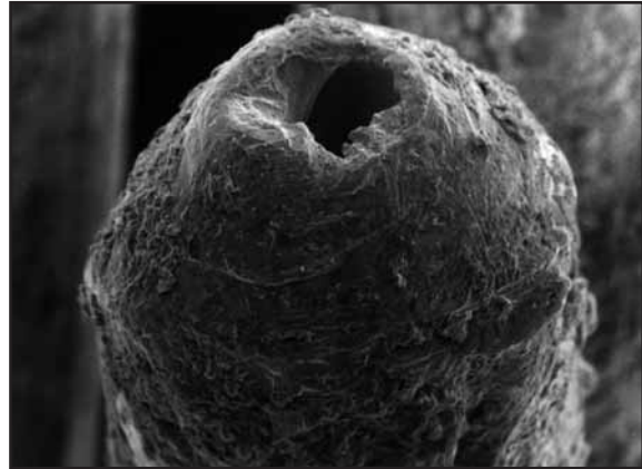
Fig. 75: Detail of wire shown in the top right of Fig. 74. Here, the temperature was even high enough to melt the wire.
