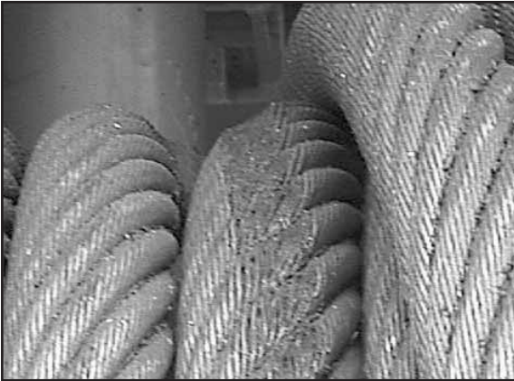
Fig. 132: This rope has made only one lift! The highly tensioned rope has cut into and deformed a lower, non-tensioned layer.
