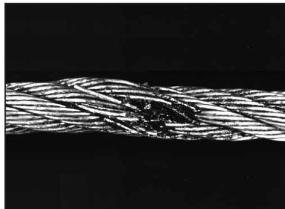
Fig. 60: Six strand rope damaged by striking a sharp edge. This rope is in a dangerous condition and must be discarded.
