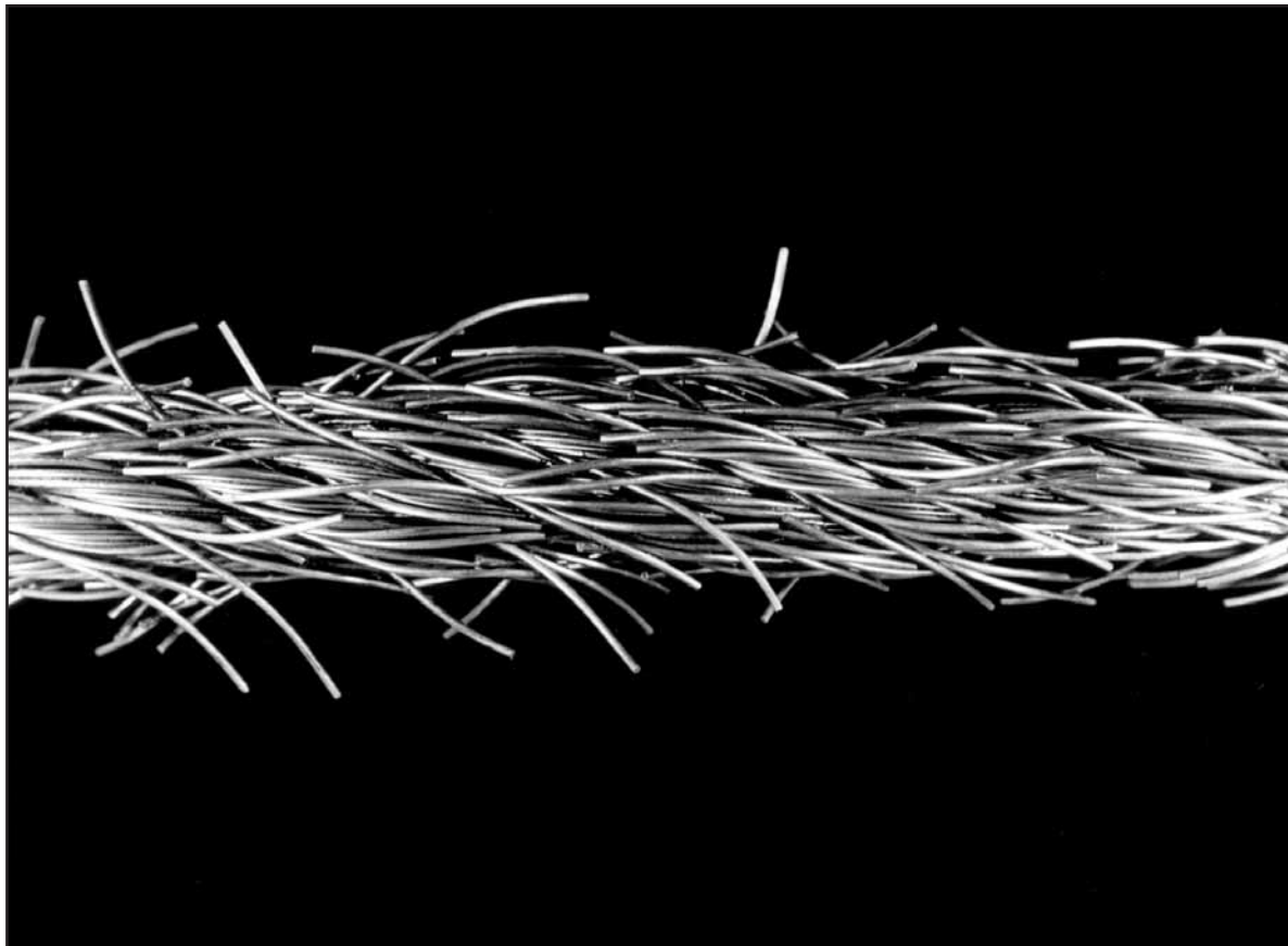
Fig. 90: This rope did not show a single external wire break. Fortunately the inspector severely bent the rope: an incredible number of internal wire breaks became apparent. A plastic layer will help prevent internal wire breaks.
