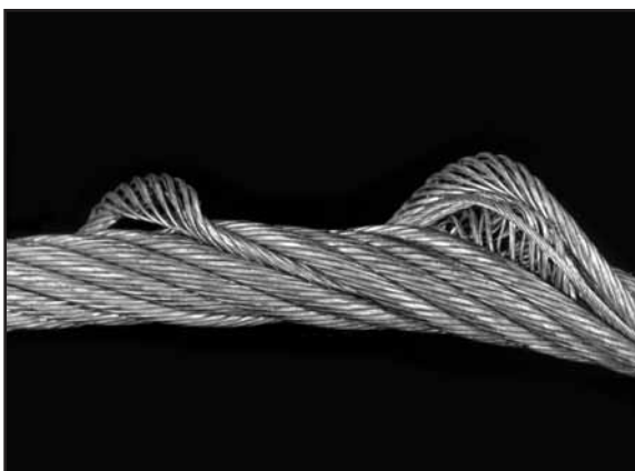
Fig. 100: Double parallel lay ropes are very sensitive to being twisted. Here the inner elements are forced out due to rope twist.
