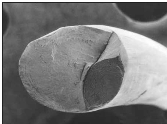
Fig. 48: A fatigue crack has propagated to a critical level before the remainder of the wire failed in shear.
