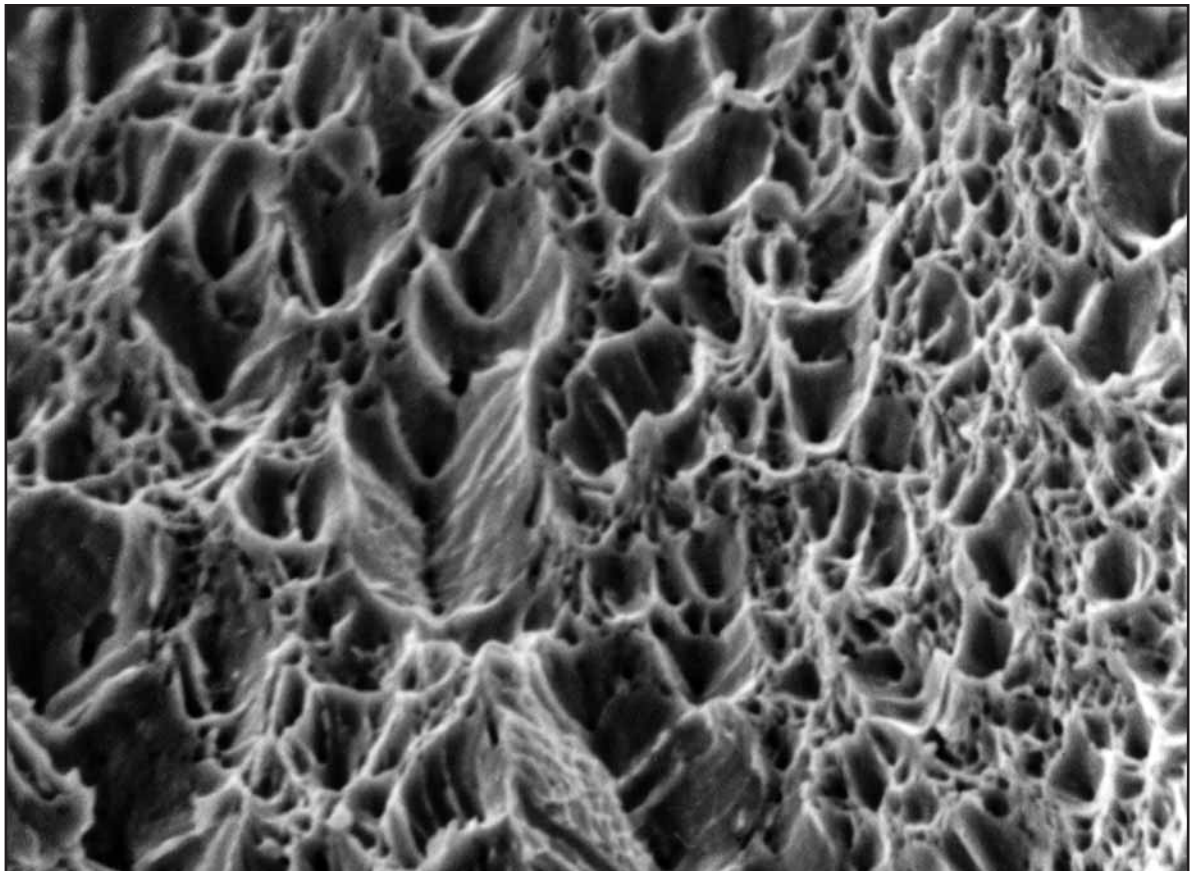
Fig. 34: Ductile dimple formations in the steel microstructure are a clear indication of a tensile overload (enlarged view of the break surface of a cone centre).
