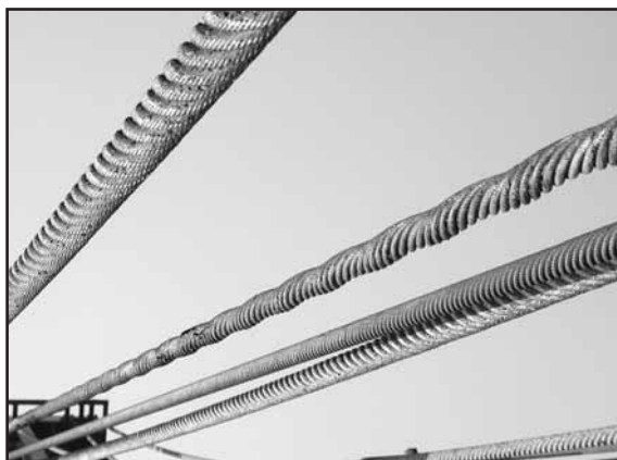
Fig. 103: Corkscrews can be formed if a rope rubs against structural members or runs through tight sheaves (a combination of rotation and friction).
