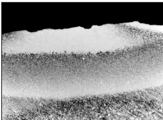
Fig. 64: Detail of Fig. 63. The white structure is martensite, the darker bands are tempered martensite.
