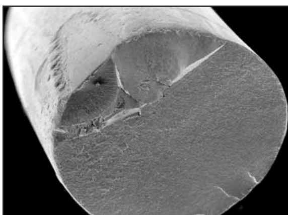
Fig. 20: A fatigue crack. The point of origin and the concentric propagation of the smaller fatigue crack is clearly visible.
