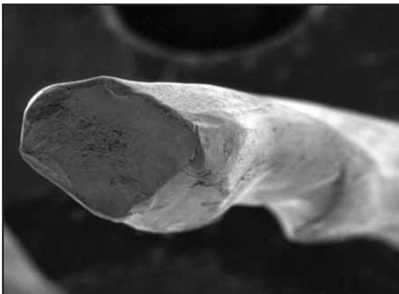
Fig. 45: Shear wire failure caused by high tensile load and interwire nicking.
