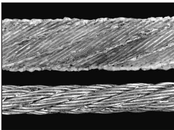
Fig. 86: Undamaged plastic coated steel core of a discarded rope after removing the outer strands and after removing the plastic layer.
