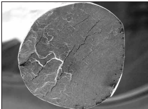
Fig. 25: Fatigue crack. The wire fatigued under the influence of both traction and compression.
