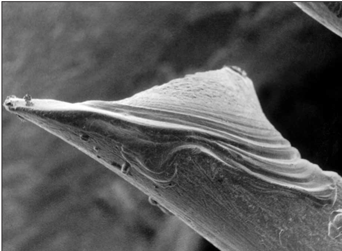
Fig. 70: A lightning strike has subjected this wire to considerable local heat causing the steel to melt.
