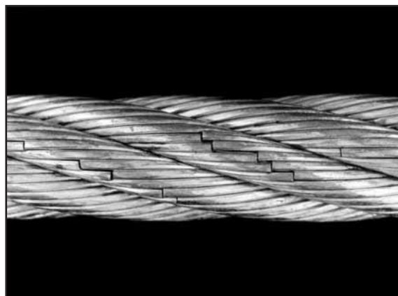
Fig. 10: This six strand rope displays almost no wear but a great number of fatigue breaks.
