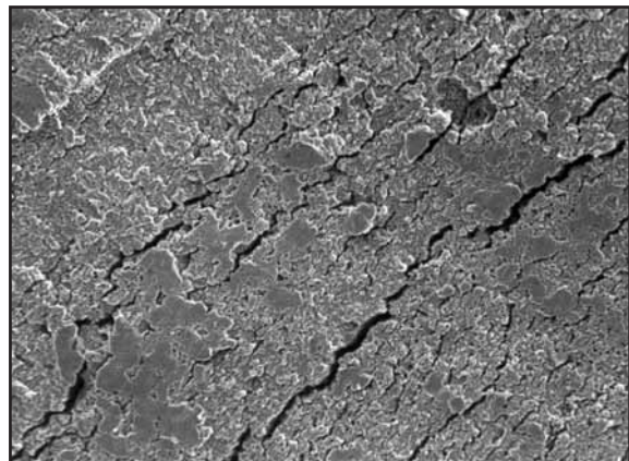
Fig. 26: Enlarged view of the crack shown in Fig. 25. The fatigue surface shows secondary deformations due to compression.
