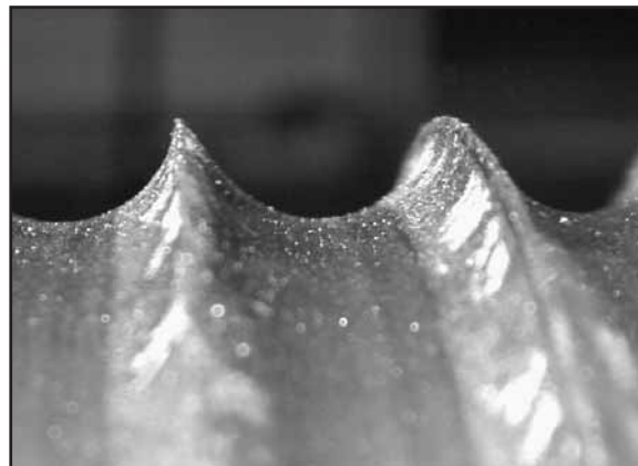
Fig. 130: If a fleet angle forces the rope fall entering the drum to rub against the groove flanges, both rope and flange might be worn.
