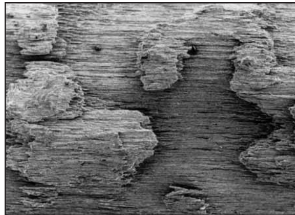
Fig. 31: The highly orientated microstructure of drawn high tensile wire becomes apparent in the corroded state.
