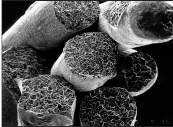
Fig. 74: The microstructure of these wires has undergone a recrystallization from the highly oriented drawn wire structure.
