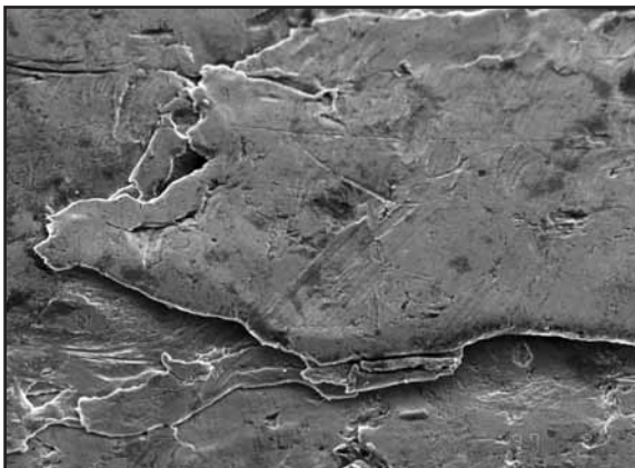
Fig. 2: Wear surface of an outer wire of a steel wire rope.
