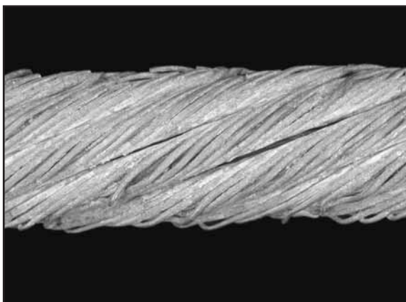
Fig. 81: Another detail of the same rope as shown in Fig. 80. Please note that the lubricant has completely disappeared.
