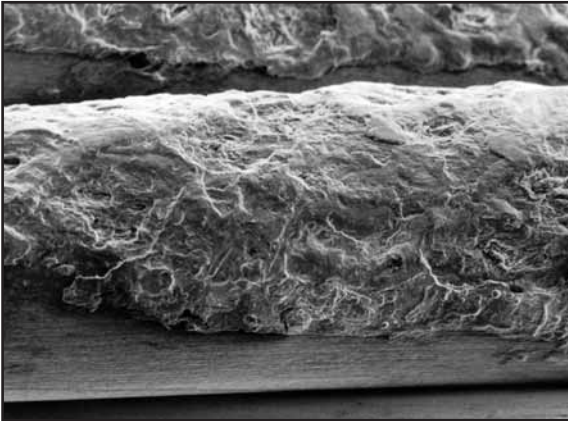
Fig. 28: Surface corrosion. Please note the increase in the effective diameter of the wire.
