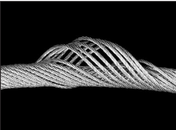
Fig. 109: Birdcage on a rotation resistant rope. If you’ve seen one you’ve seen them all.
