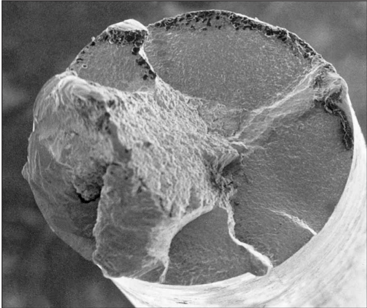
Fig. 24: Wire fatigued in rotary bending fatigue test. The cracks initiate from all around the circumference.
