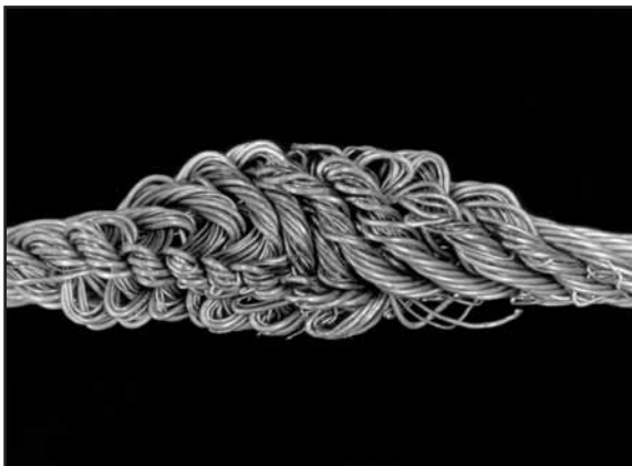
Fig. 98: This shows the rope section from Fig. 97 with the outer stands removed to reveal the surplus length accumulated in the core.
