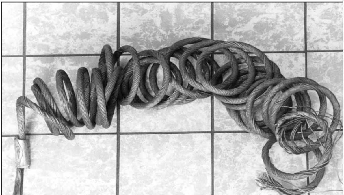
Fig. 62: Ropes that have been pulled over a sharp edge have a tendency to coil when unloaded.
