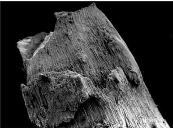
Fig. 30: Tensile failure of a wire weakened by corrosion.
