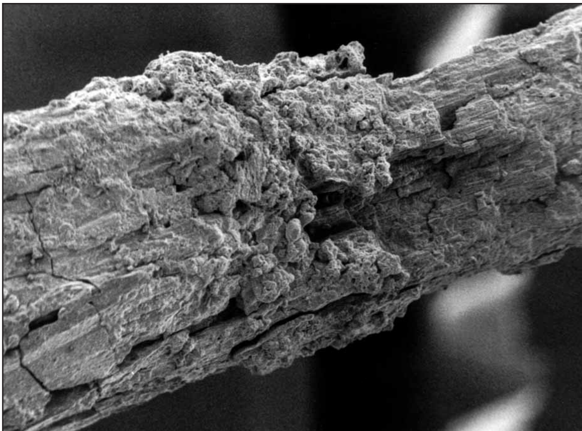
Fig. 27: Severe uniform corrosion (atmospheric corrosion). Static ropes and ropes operating in a marine environment should be galvanized and well lubricated. A plastic coating between the steel core and the outer strands will protect internal rope elements.
