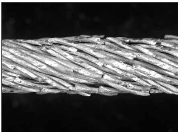
Fig. 88: The rope core shown in Fig. 87 after removing the plastic layer. The outer wires have broken at the crossover points.
