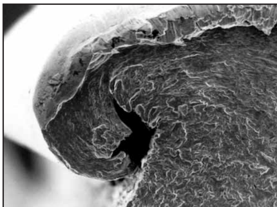
Fig. 7: Plastic wear on the surface of an outer wire. The material displacement is very visible.
