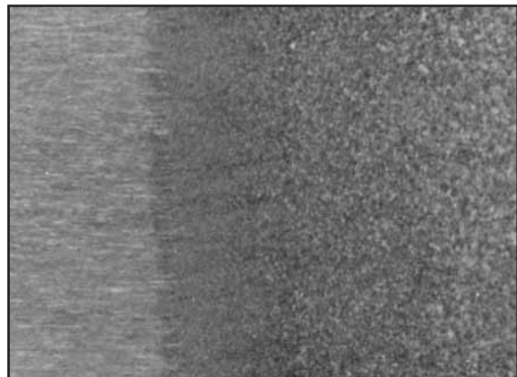
Fig. 79: This etched sample shows the transition from the cold drawn wire structure (left) to the recrystallized structure (right).
