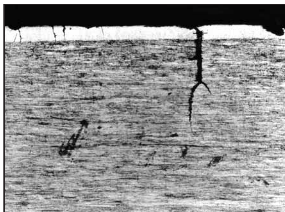
Fig. 67: Detail of Fig. 66 showing the crack formation.
