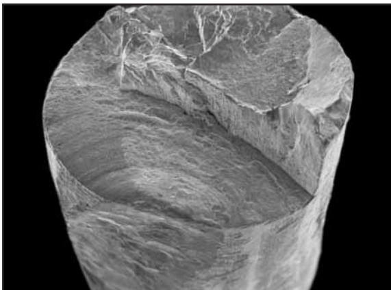
Fig. 16: A fatigue crack.
