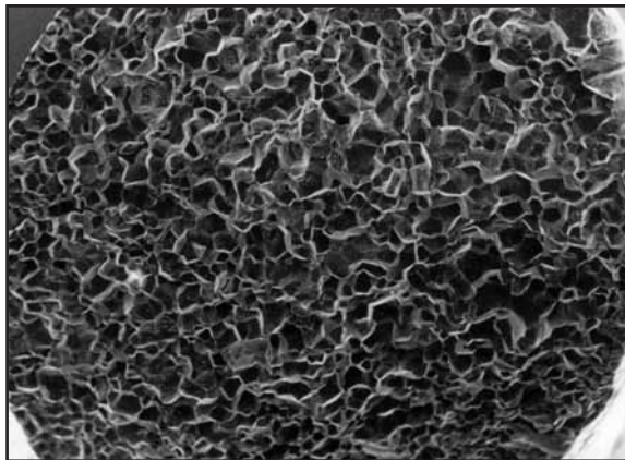
Fig. 76: Recrystallized structure.
