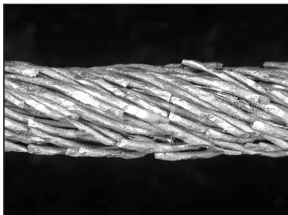
Fig. 89: The rope core shown in Fig. 87 after removing the plastic layer. The outer wires have broken at the crossover points.
