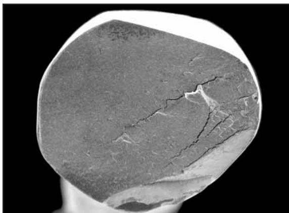
Fig. 18: If the line pull on a fatiguing wire is low (high design factor), the area affected by fatigue before final failure is large.
