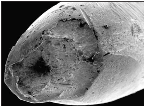
Fig. 38: Cup and cone tensile failure at a crossover point.
