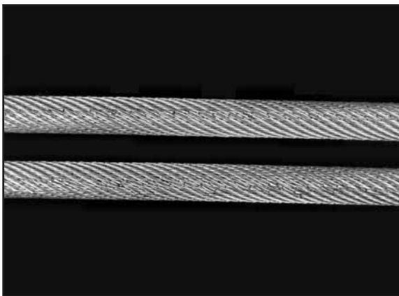
Fig. 114: This rope has operated in a groove which was much too wide, leading to premature wire failure along the line of contact.
