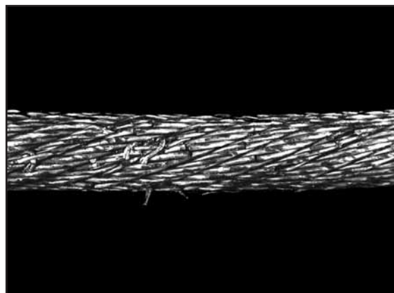
Fig. 92: The same 36 x 7 rope after removing the outer strand layer. Many wire breaks can be found at the crossover points.
