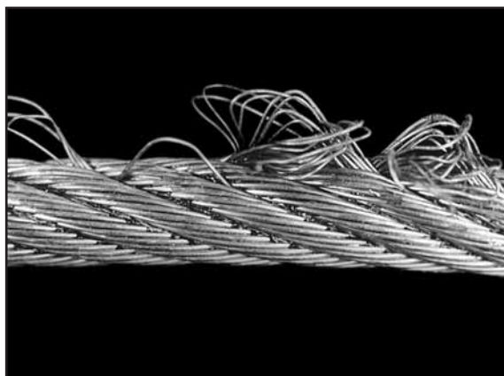
Fig. 145: An incorrect backtwist in the rope closer has shortened the strands. The inner wires were then be under compression and later popped out.
