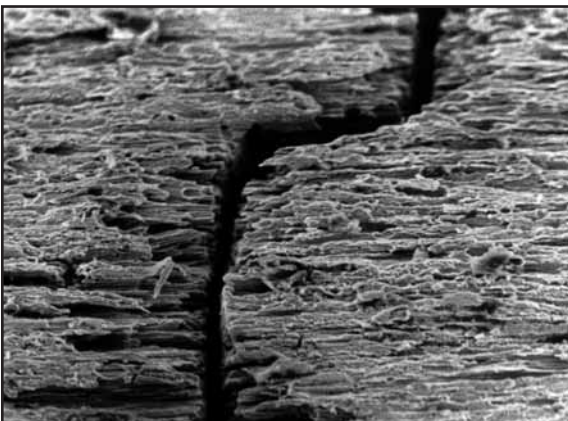
Fig. 32: Stress corrosion crack. Tensile stresses help propagate a crack initiated by corrosion.
