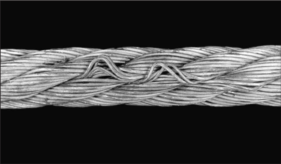
Fig. 141: Loop formations can be (but may not be) caused by insufficient clearance between the wires in the strand. Lack of clearance will prevent these wires from moving relative to their neighbours, causing overloading and yield.
