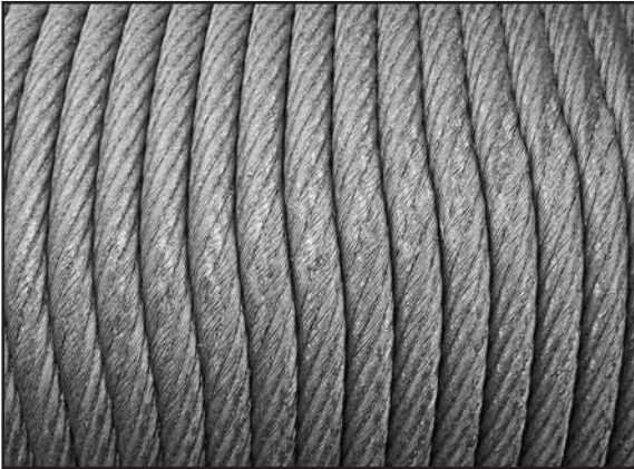
Fig. 125: Inclined wear pattern in multi layer spooling normally indicates an incorrect rope diameter.
