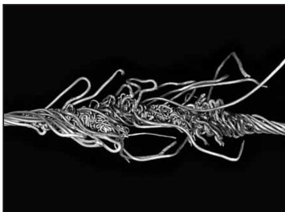
Fig. 101: Sometimes the rope twist only affects the innermost strand which is the shortest and the only straight strand in the rope.
