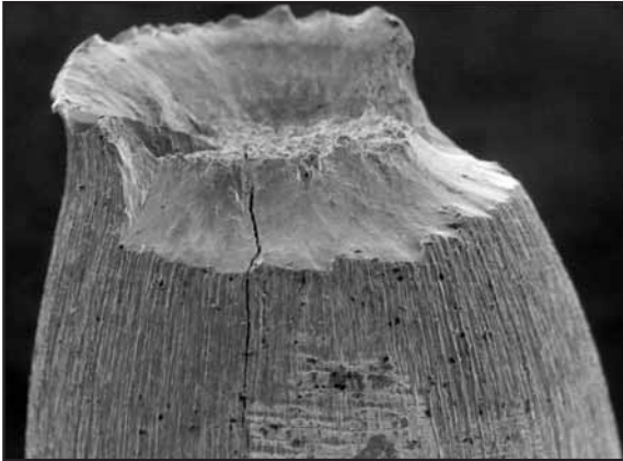
Fig. 35: Classic cup and cone tensile failure. Half of the end has a cup shape and half has a cone shape.
