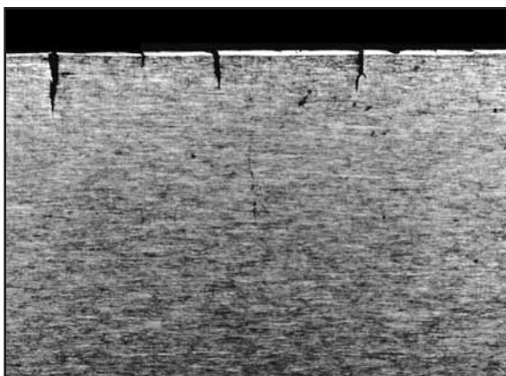
Fig. 66: Layer of martensite on the surface of a rope wire.
