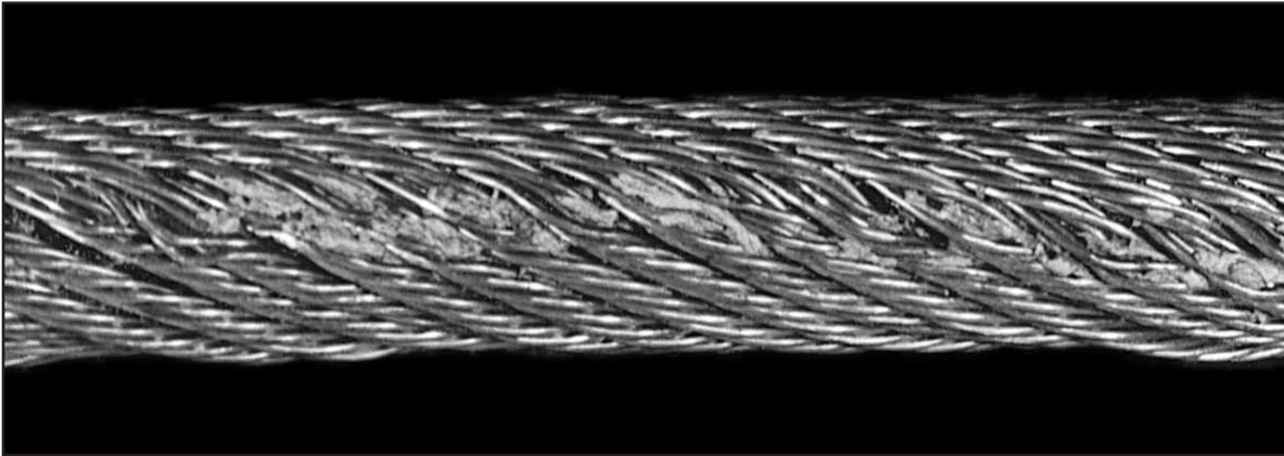
Fig. 119: This rope has “jumped” a plastic sheave. Please note the plastic particles in between the outer wires. Due to the higher coefficient of friction, under otherwise similar conditions, a rope will “jump” a plastic sheave earlier than a steel sheave.
