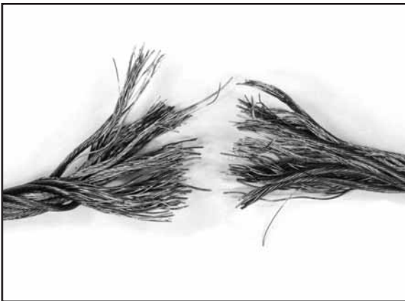
Fig. 120: A rope which has failed having “jumped” a sheave will often look as if it has been cut by an axe (shear and tensile failures).
