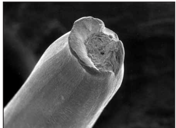
Fig. 43: Oh yes, another tensile overload break.
