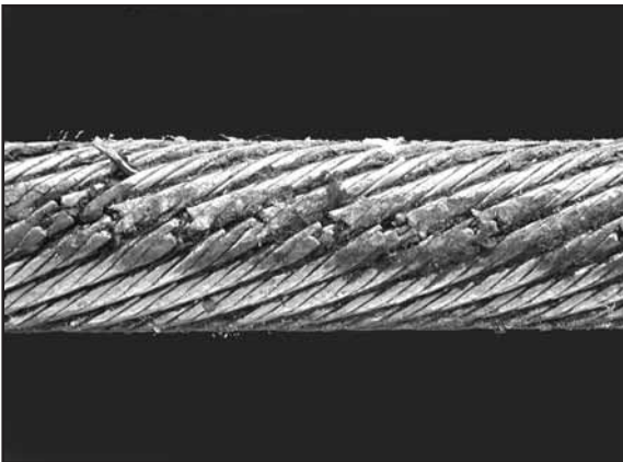
Fig. 127: Typical rope damage created in the cross over zone.
