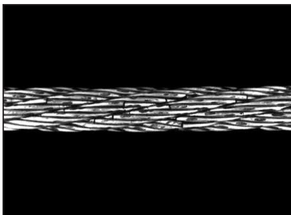
Fig. 93: The innermost strand layer of the same 36 x 7 rope also shows a great number of wire breaks.
