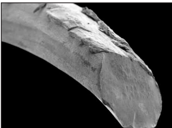
Fig. 47: High transverse loading initially caused severe plastic wear. Finally the wire failed in shear.
