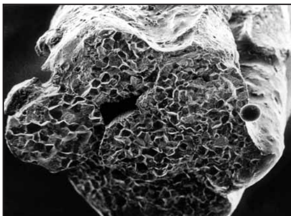
Fig. 72: At even higher temperatures, the steel will melt and the individual wires fuse.
