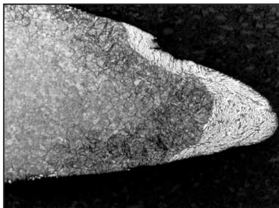
Fig. 65: Martensite (white tip) formed by arcing.
