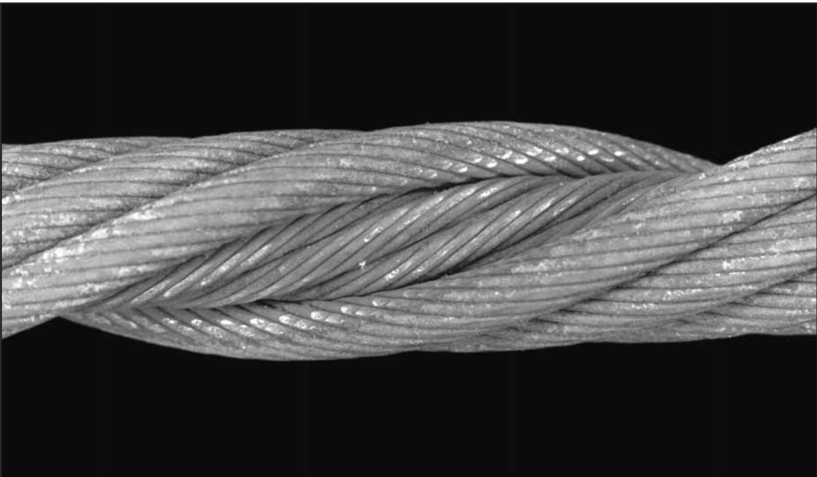
Fig. 142: If the diameter of the steel core of the rope is too small, the outer strands will not have sufficient clearance. Interstrand nicking will occur. Lack of clearance will considerably reduce the rope's fatigue life.
