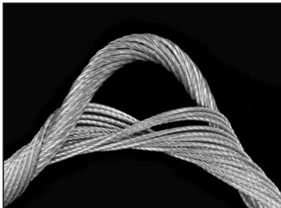
Fig. 99: This rotation resistant rope has been shortened, and its core lengthened, by twisting the rope in the closing sense.
