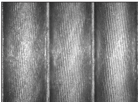
Fig. 95: Longitudinal scratch marks on a drum suggest that the rope might develop internal wire breaks.
