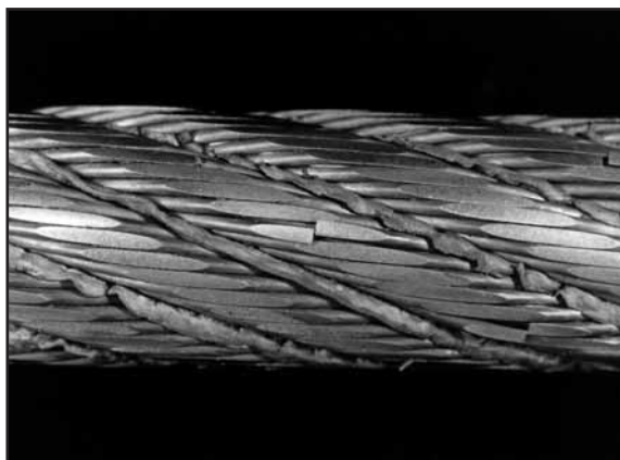
Fig. 9: Heavily worn wire rope with a few fatigue breaks. The wire ends are displaced in different directions because of rope twist.
