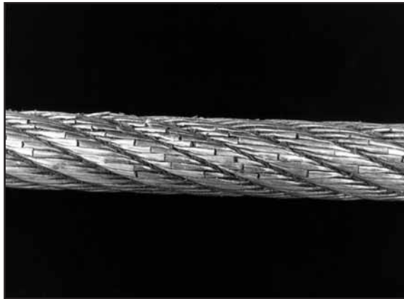
Fig. 113: Another example of a rope which has worked in a tight sheave.
