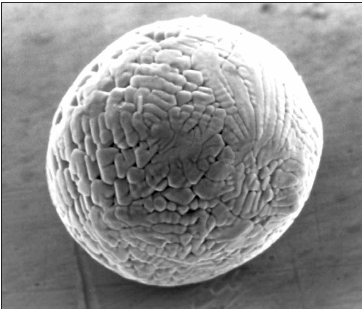
Fig. 138: Manganese- Sulphite balls in the wire structure are extremely hard and do not deform in the wire drawing process. They often appear on the surface of fatigue breaks because wires will tend to fail in sections already weakened by such inclusions.
