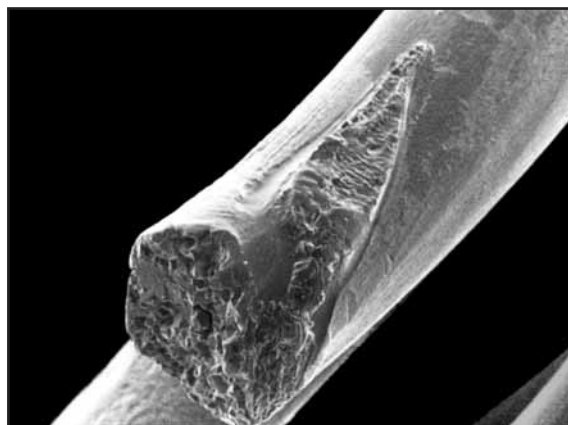
Fig. 73: The recrystallization is accompanied by an increase in volume, causing the wire to crack longitudinally.
