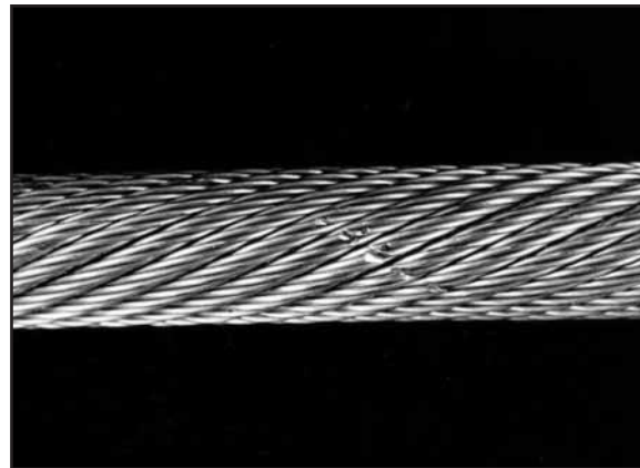
Fig. 58: Rotation resistant rope damaged by striking a sharp edge.
