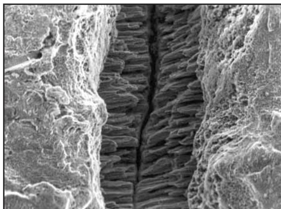
Fig. 69: Detail of the same wire as shown in Fig. 68. A fatigue crack has formed underneath the zinc coating.
