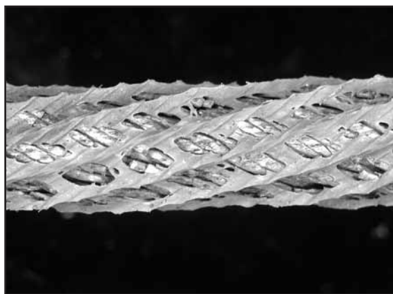
Fig. 87: Damaged plastic layer perforated by the outer and inner strands. The hardness of the plastic was insufficient for the purpose.
