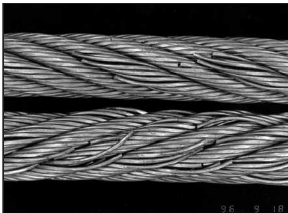
Fig. 84: The great number of internal wire breaks have only been revealed by severely bending the ropes during inspection.
