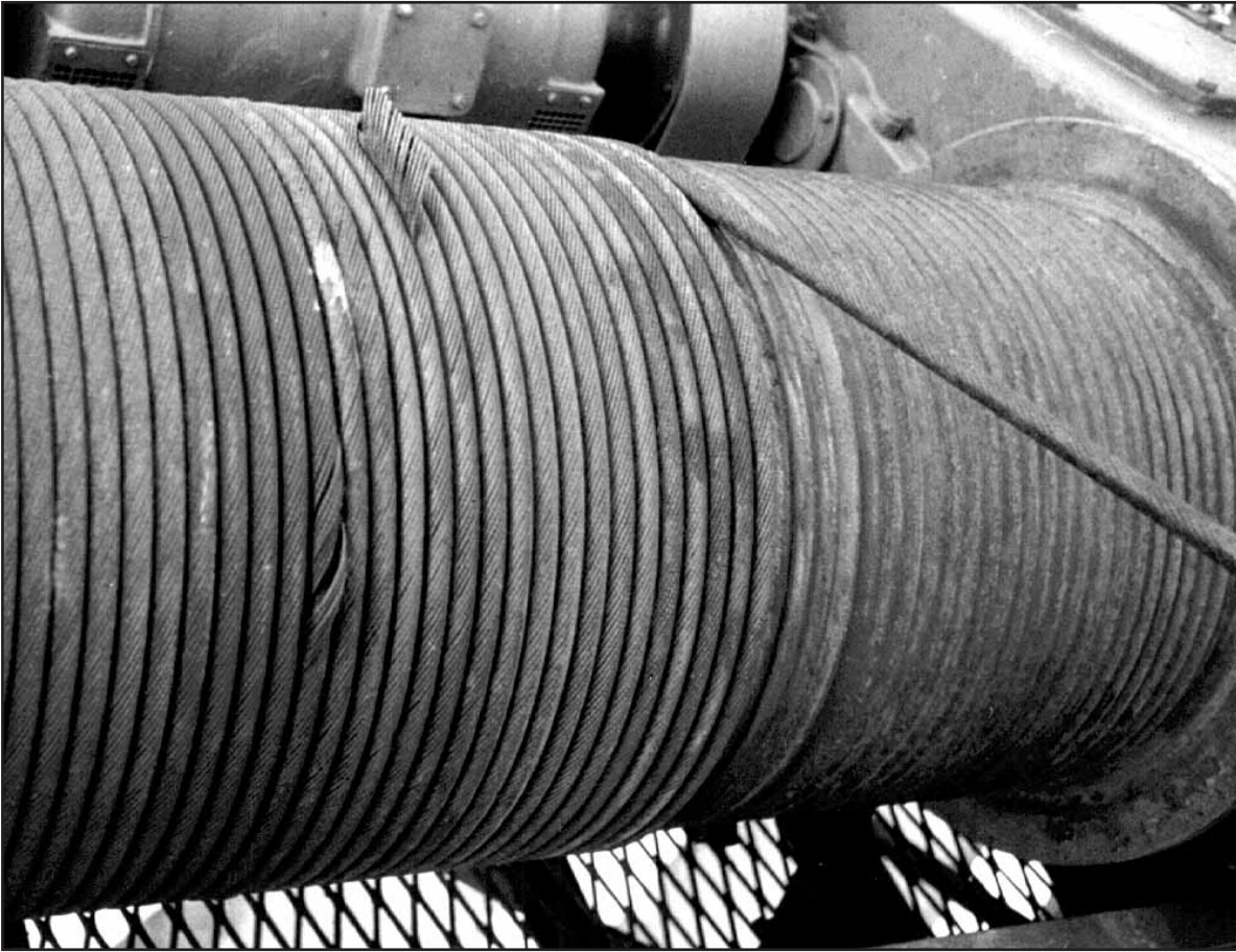
Fig. 108: This semi rotation resistant rope has been attached to a free spinning swivel. Under load, the rope opened up, and twisted rope sections travelled through the reeving system. The sheaves moved the “superfluous” strand lengths through the reeving system until they ended up on the drum. This is a typical example of how an action at one end of the rope (the use of swivel) causes a reaction (the creation of birdcages) at the other.
