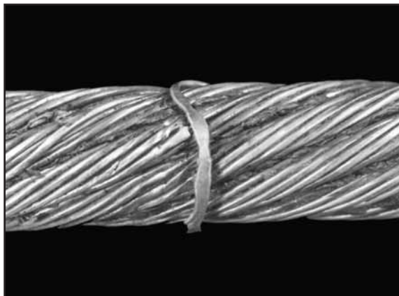
Fig. 117: Across strand nicking damage is especially relevant to Langs lay ropes where the exposed wire ends are always long.
