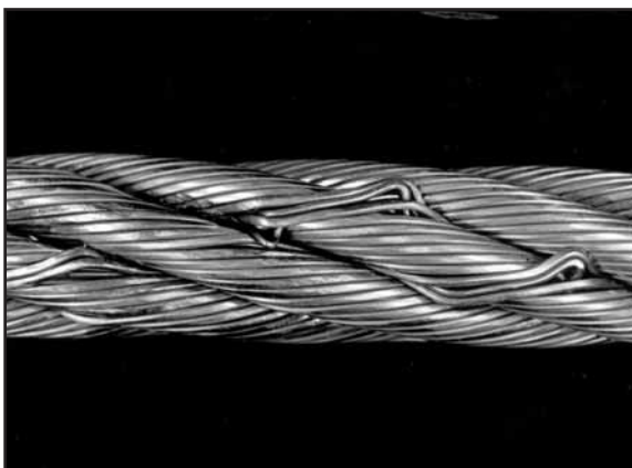
Fig. 102: In this six strand rope, twist has loosened the two outer layers of wires in the outer strands.
