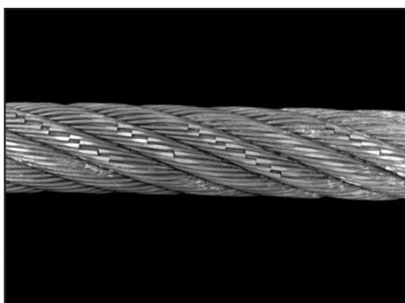
Fig. 11: Three adjacent strands with fatigue breaks followed by one without indicate uneven load sharing or a pulled-in strand.
