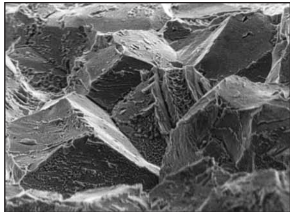
Fig. 77: This detail of Fig. 76 shows the intergranular fracture of the crystalline structure.
