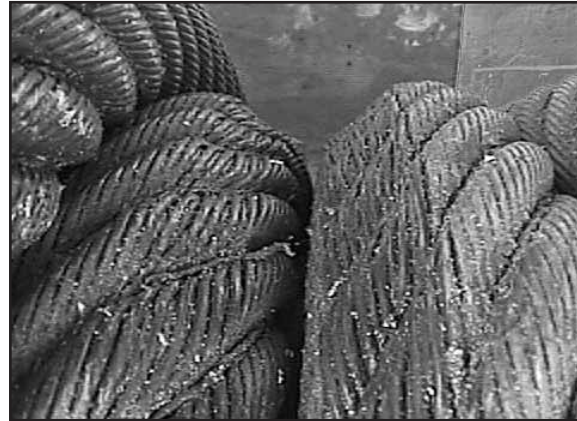
Fig. 133: This rope, too, has only made one lift! Again, lack of pretension caused the rope damage.
