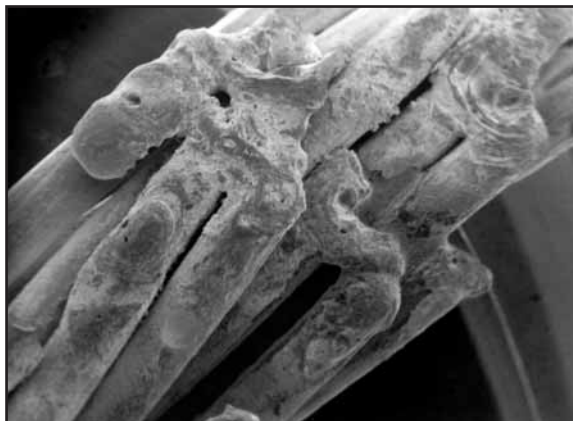
Fig. 78: High local temperatures during arcing fused these wire ends.
