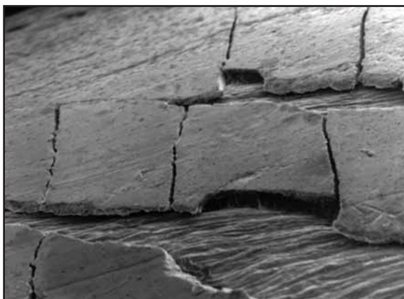
Fig. 68: No, this is not martensite. It is the zinc coating of a galvanized wire flaking off (see also Fig. 111.)
