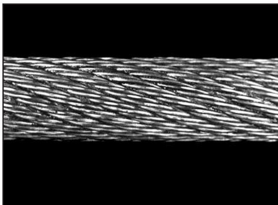
Fig. 91: Outer surface of a 36 x 7 rotation resistant hoist rope. No wire breaks are visible.
