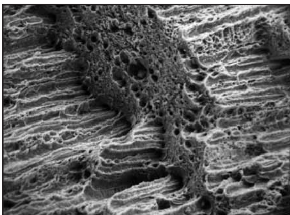
Fig. 139: The fracture zone of a wire destroyed through severe bending (very low cycle fatigue) will look like split wood.
