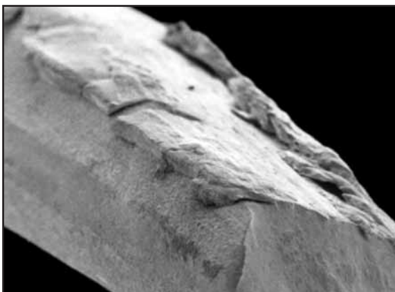
Fig. 6: Plastic wear on the surface of an outer wire. Cracks will initiate at the work hardened surface.
