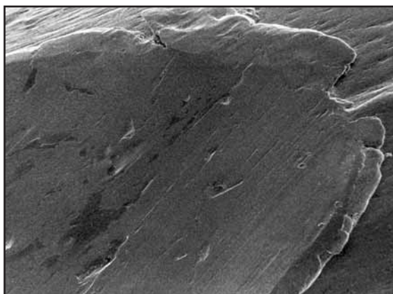
Fig. 5: Plastic wear of a rope wire at a cross-over point inside the rope. The cold-working will harden the material and form cracks.
