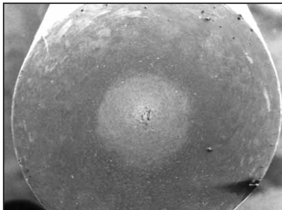
Fig. 140: The fracture surface of a rope wire destroyed by pure torsion will look like an old 33 rpm LP record.
