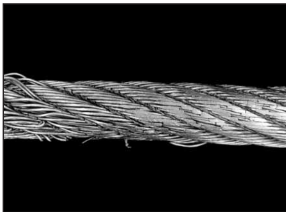
Fig. 115: This rope has been dragged over a stuck sheave. Note severe abrasion to the right and loose wires to the left.
