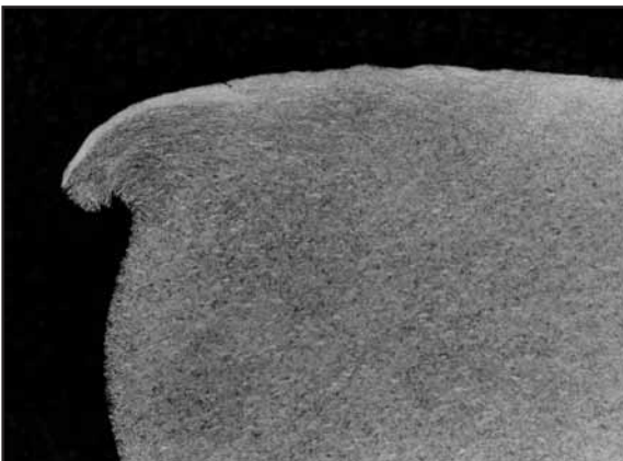
Fig. 129: Abrasion and plastic wear (see page 4) caused by rubbing against a neighbouring rope wrap (see Fig. 128).
