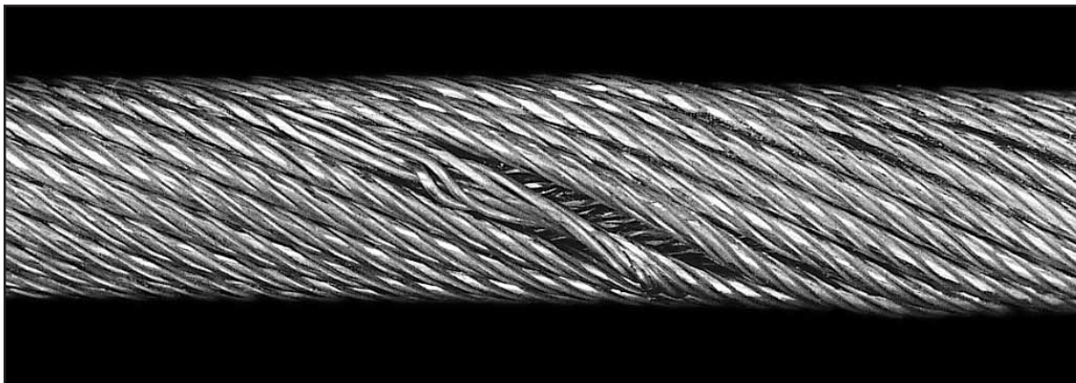
Fig. 143: During stranding, one strand obviously had slipped on the capstan, locally creating a long lay length. This stranding defect was not detected before the faulty strand was closed into the rope.
