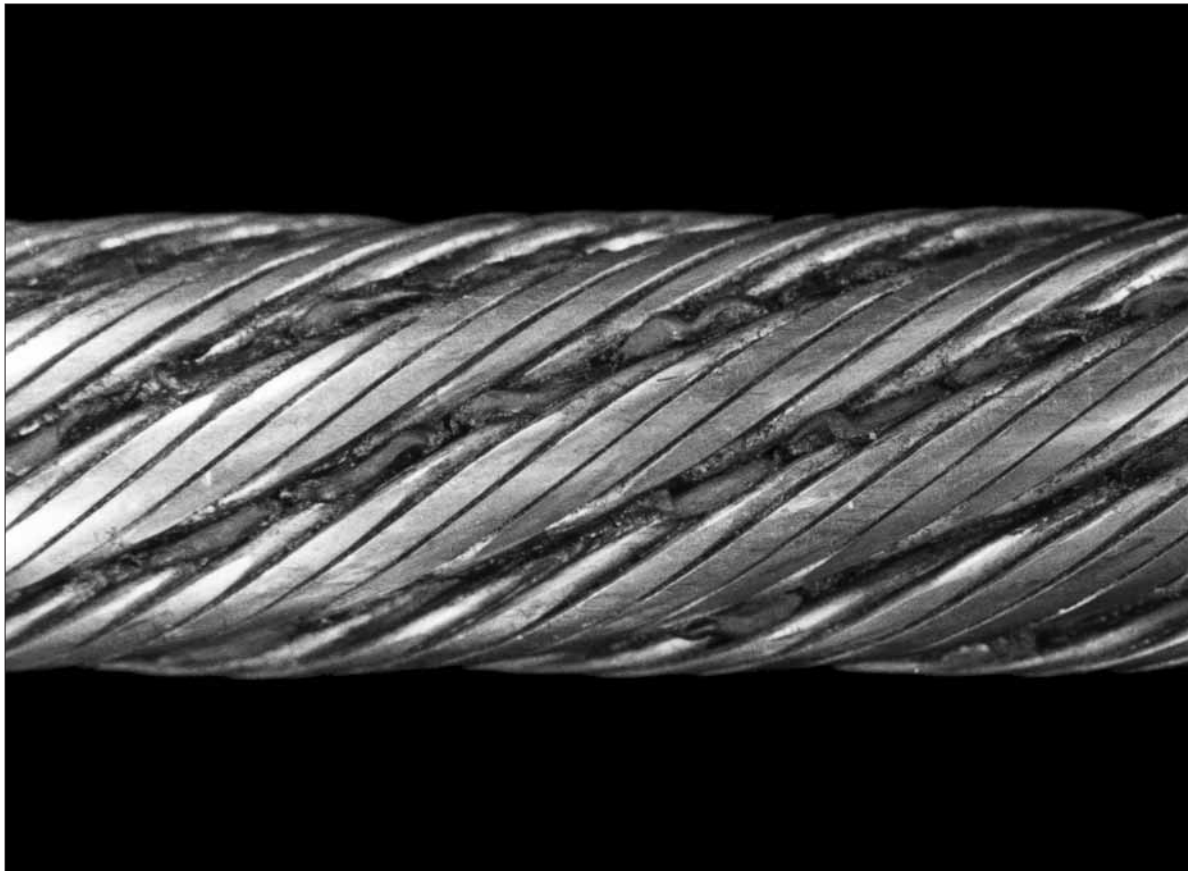
Fig. 1: A Langs lay rope with a great amount of uniform mechanical wear. Please note that the rope does not exhibit any fatigue breaks. The bearing surface on sheaves and drums has increased due to the mechanical wear.
