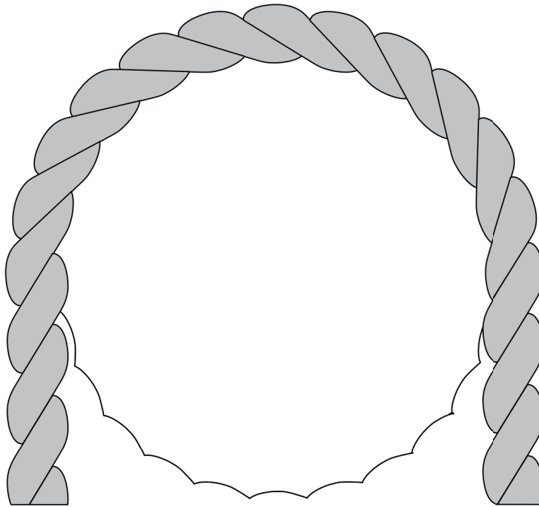
Fig. 5: Good contact conditions for the old rope
