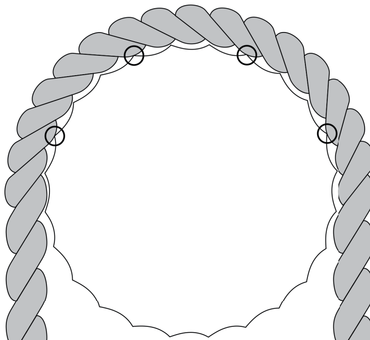
Fig. 6: Very bad contact conditions for the new rope
